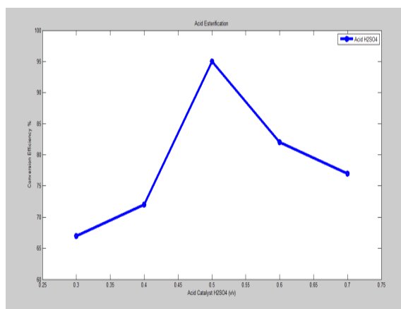
Fig. 2. Effect of acid Catalyst Amount on Conversion Efficiency
