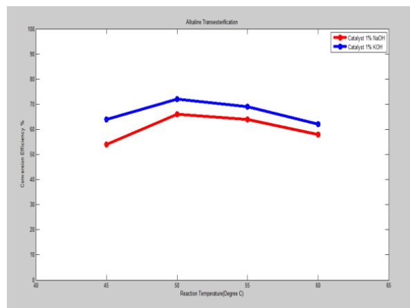
Fig. 5. Effect of Reaction Temperature on Conversion Efficiency
