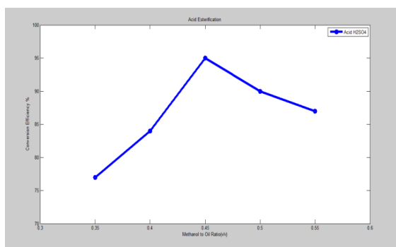
Fig. 1. Effect of Methanol-to-Oil Ratio on Conversion Efficiency
