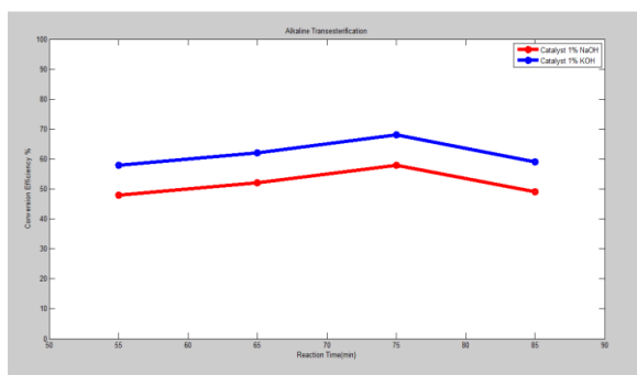
Fig. 6. Effect of Reaction Time on Conversion Efficiency
