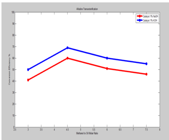
Fig. 3. Effect of Methanol on Conversion Efficiency
